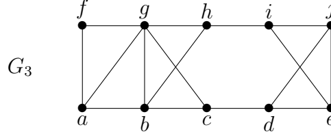
Figure 4: G_3 is not AT-free, (g, i, d) is an AT, but G_3 is 1-strongly laminar.
