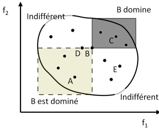
Figure 1.14 – Illustration des relations de dominance entre solutions
