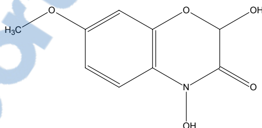
FIGURE 8 : Benzoxazinone
