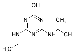
Hydroxy-atrazine
