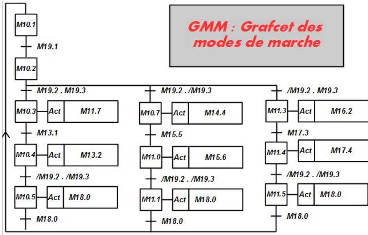
Figure 43: GMM niv 1
