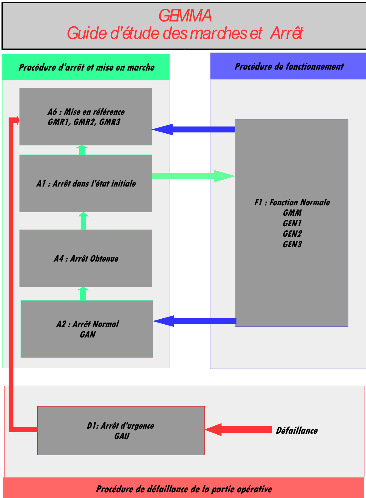
Figure 19: GEMMA
