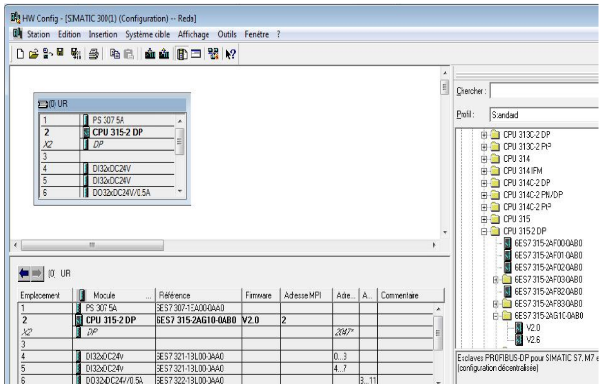
Figure 41: Configuration matérielle
