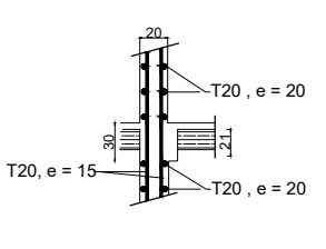
Coupe 8'-8'
