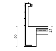
Coupe 2'-2'
