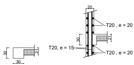
Coupe 1'-1'
