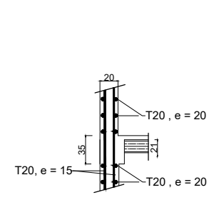
Coupe 2'-2'
