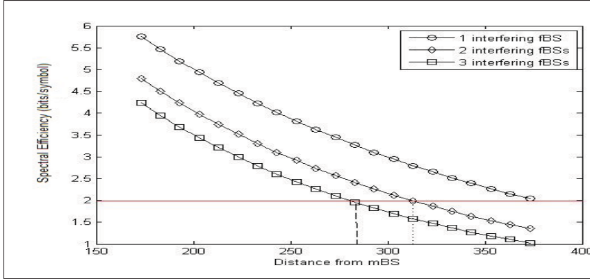
Figure 3.2 Achievable spectral efficiency in MC zone Z_3
