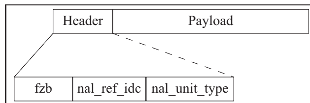
Figure 1.3 Composition of a Network Abstraction Layer Unit
