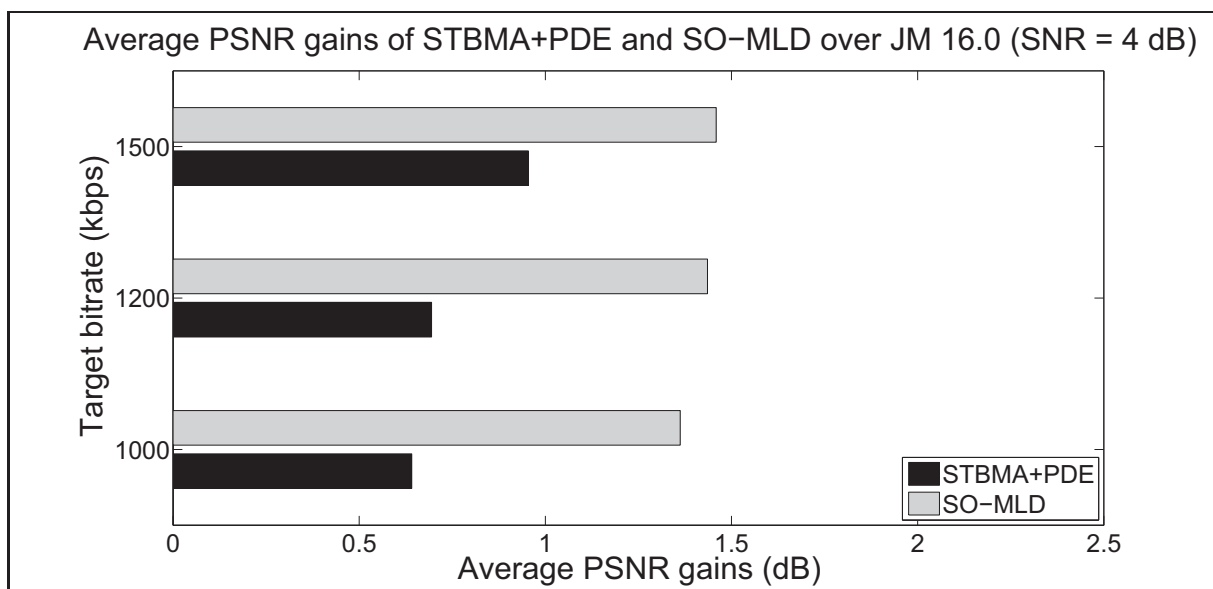
Figure 5.2 Average PSNR gains of STBMA+PDE and SO-MLD over JM 16.0 when the channel SNR is 4 dB
