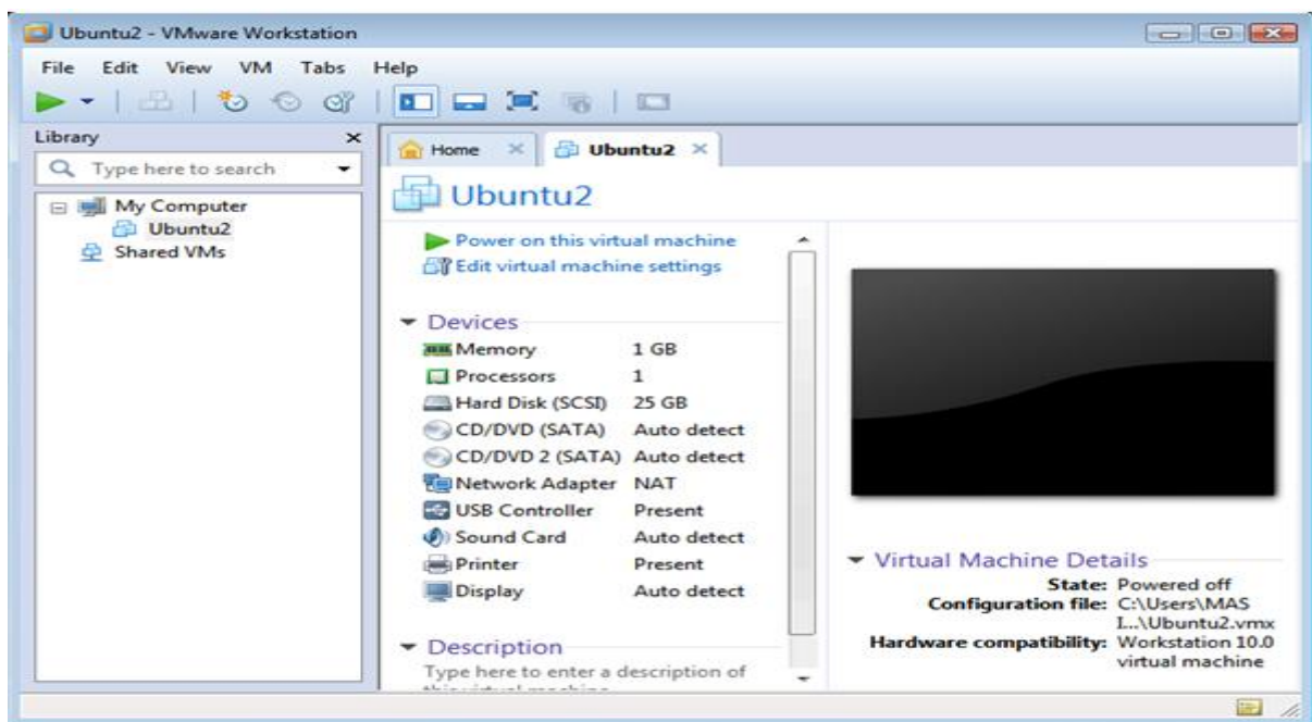
Figure III-2 : Machine VMware.
