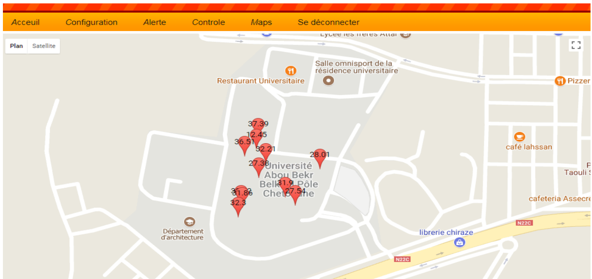
Figure IV-19 : page Map.
