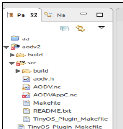
Figure III-24 : Package AODV
