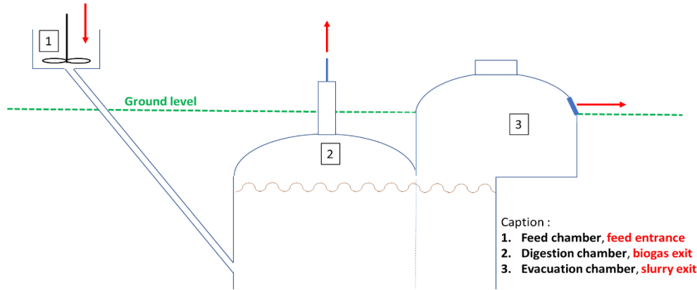
Figure 1: Showing the configuration of a fixed dome digester.
