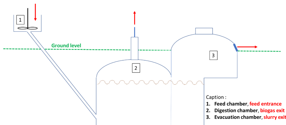
Figure 1: Showing the configuration of fixed dome digester.
