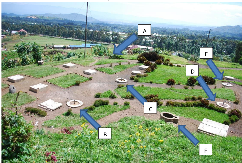
Figure 1 : 4x100m 3 digesters installation in RUBAVU prison.
