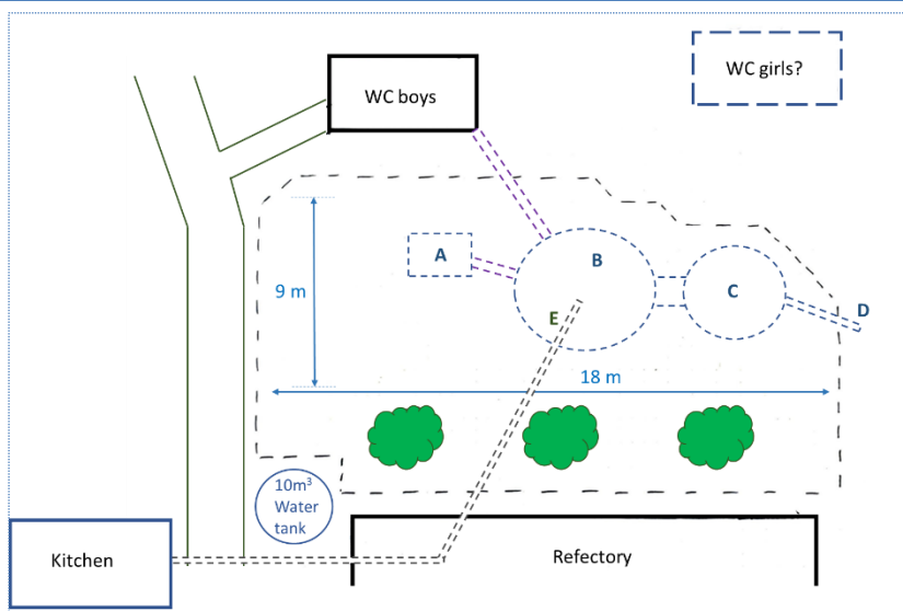
Figure 3: site for the digester, after construction.
