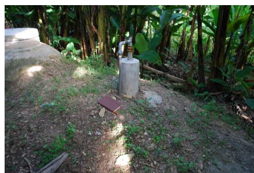
Figure 2: digester chamber, with gas tap on the top. On the back left, evacuation chamber.
