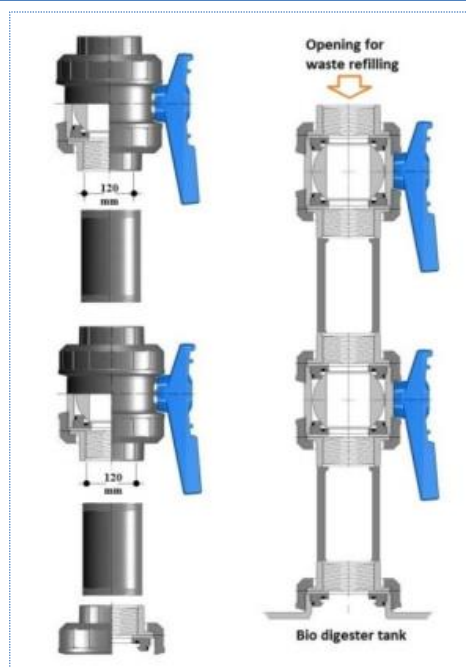
Figure 4: double valve system proposed to prevent entry of oxygen, loss of biogas and rise of unpleasant odour. [14]
