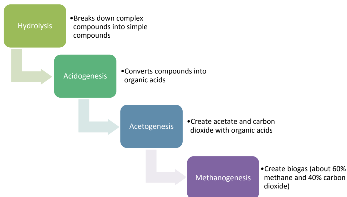
Figure 1 : key steps of anaerobic digestion.
