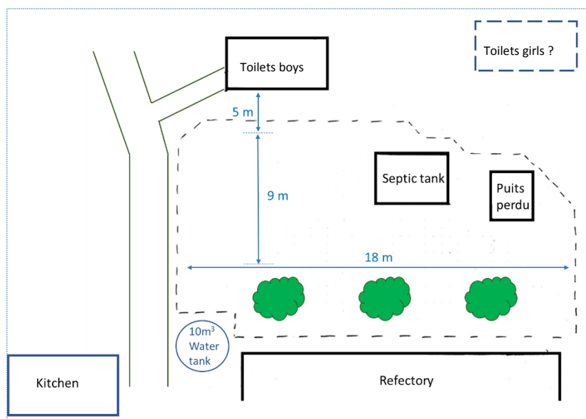
Figure 2: selected construction site for the digester, before construction.
