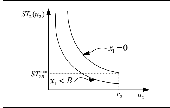
Figure 3.5 Characteristic of the time saved of M_2 .
