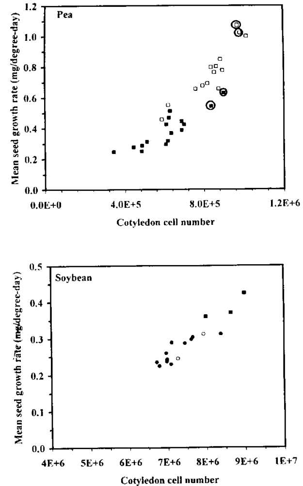
Fig. 3. The relationship between cotyledon cell number and seed growth rate. Pea: Frisson (■) and Solara (□), in various environmental conditions. Circles denote seeds from depodded plants. Soybean: 1991, 20 plants m -2 (●), 1991, 80 plants m -2 (○), 1992, 20 plants m -2 (■): for each symbol, different points correspond to different morphological positions within the plant.
