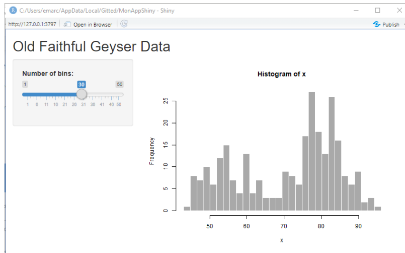
FIG. 7.1 : Application Shiny Old Faithful Geysers Data.
