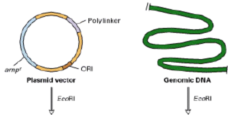
(b) Insertion of EcoRI restriction fragments
