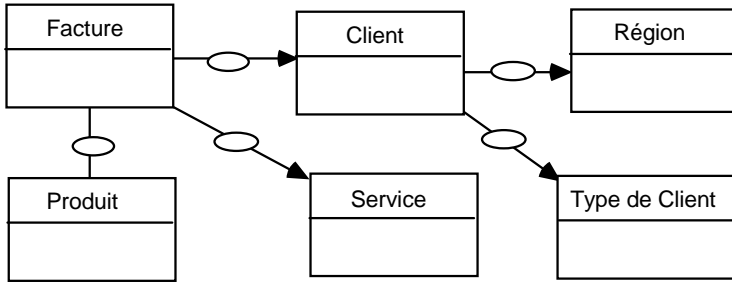
MCD "Production"
