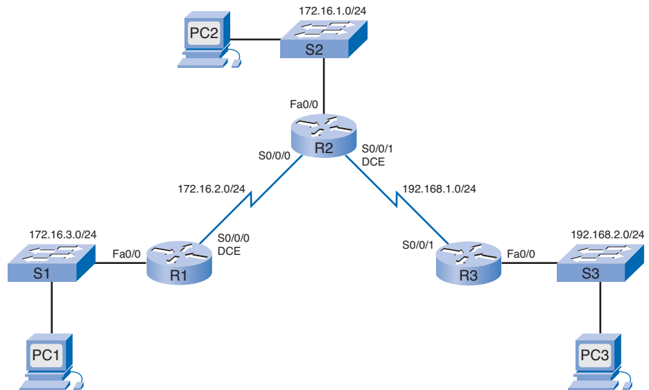
Figure 3-11 Administrative Distances and Static Routes
