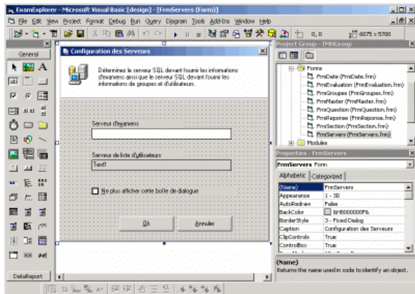
Figure 1.3 – Visual Basic 6.0
