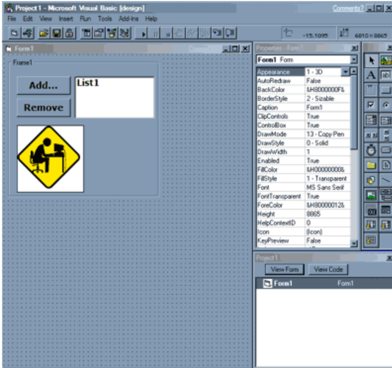
Figure 1.2 – Visual Basic 4.0
