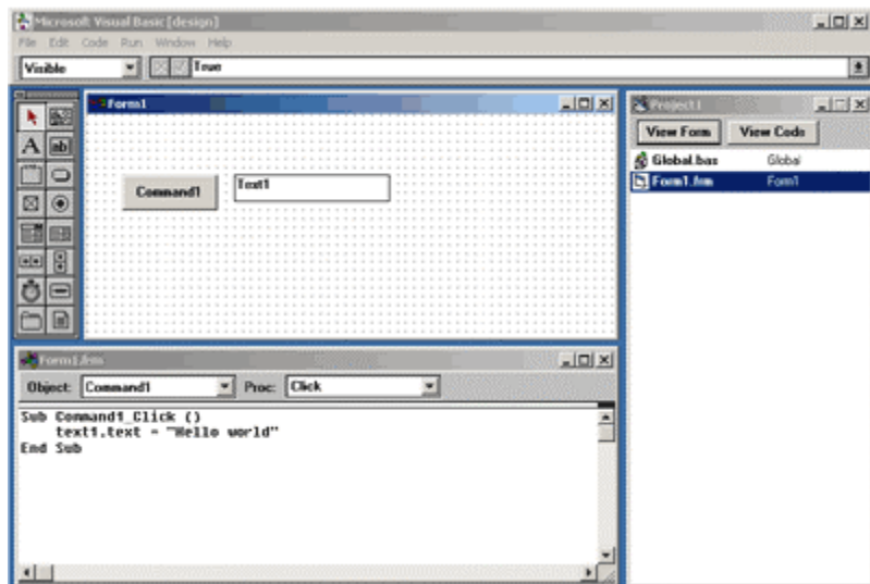
Figure 1.1 – Visual Basic 1.0
