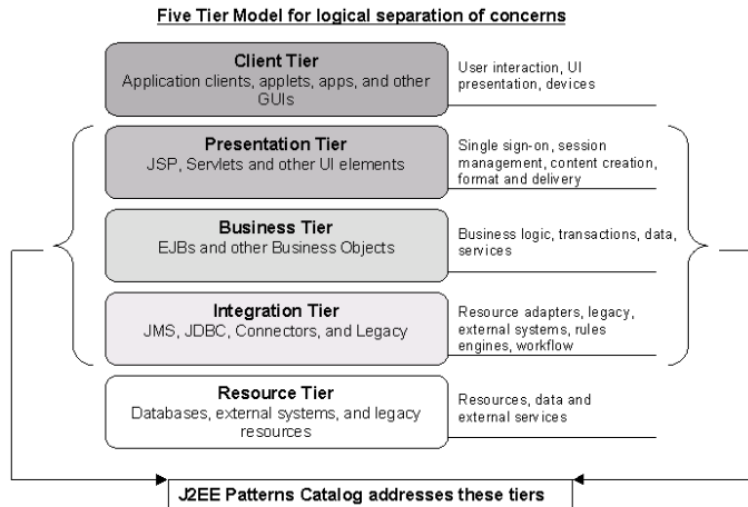
Fig.: Architecture J2EE 5-tier
