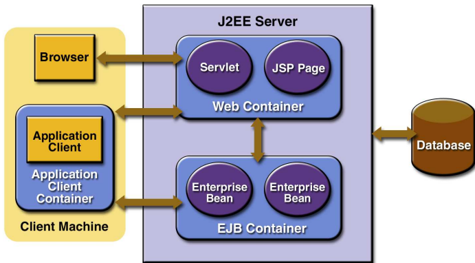
Fig.: Conteneurs J2EE
