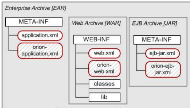
J2EE Enterprise Archive [EAR] structure.
