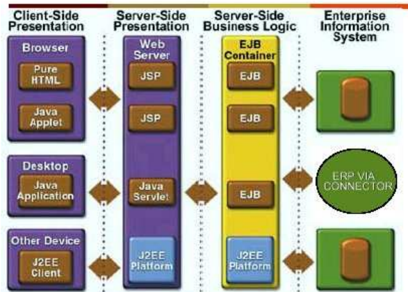
Fig.: Architecture J2EE n-tier
