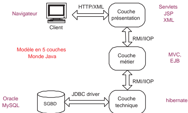
Fig.: Architecture Web simple
