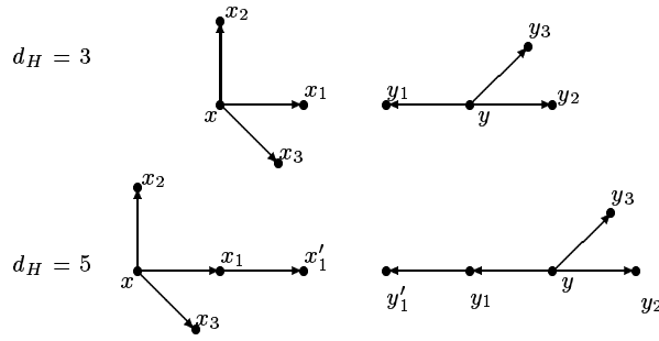
FIG. 1.14 - Distance de Hamming.
