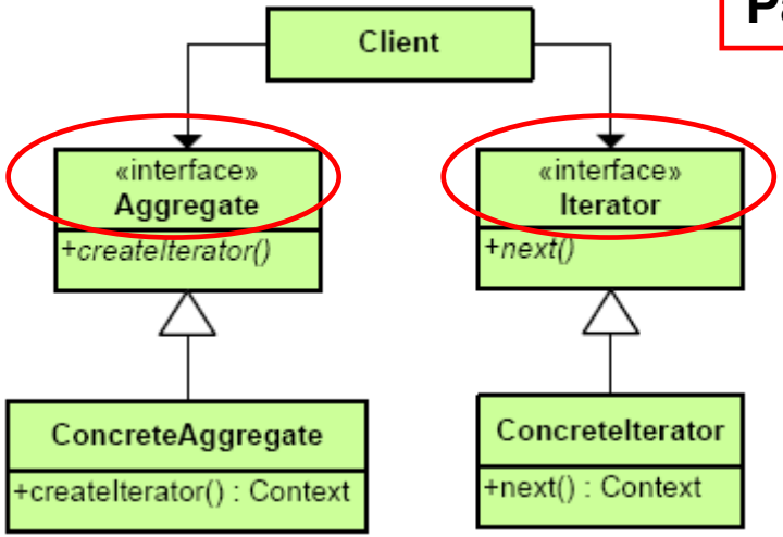
Iterator
