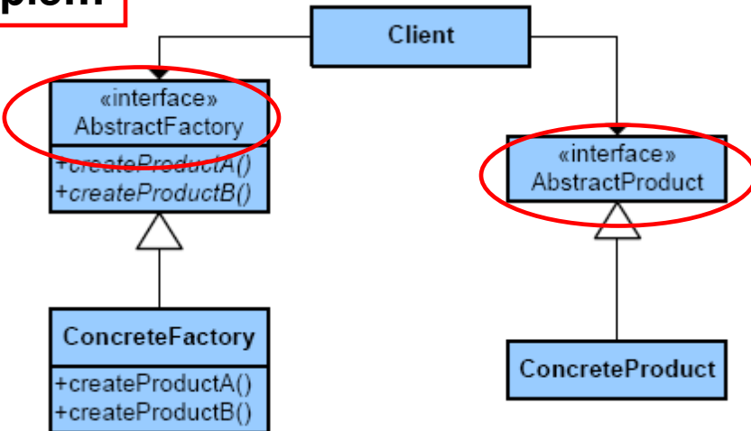
Abstract Factory
