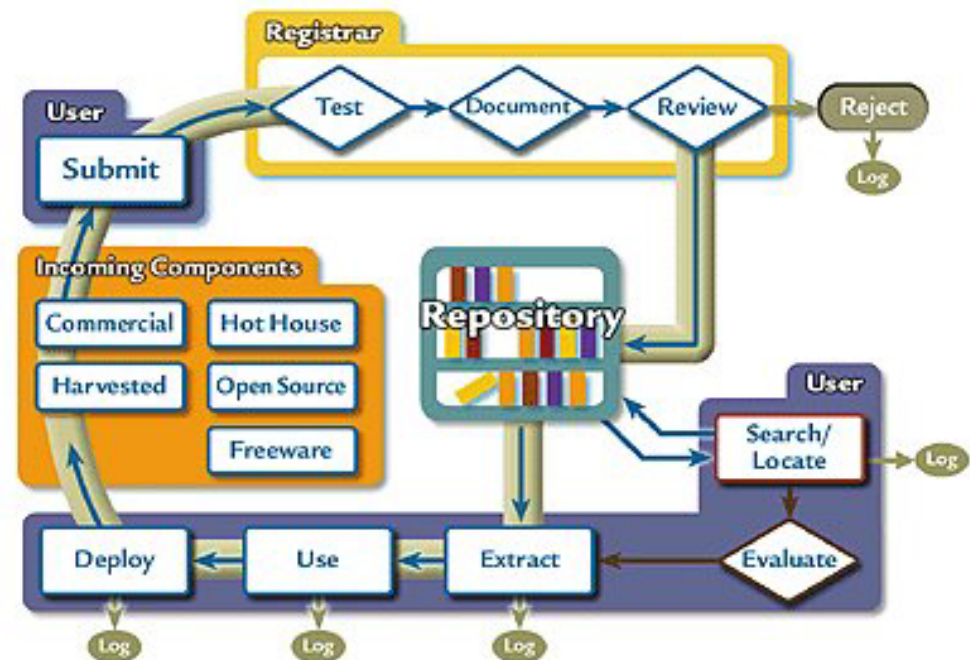
FLASHLINE COMPONENT MANAGER™ 2 REUSE OVERVIEW
