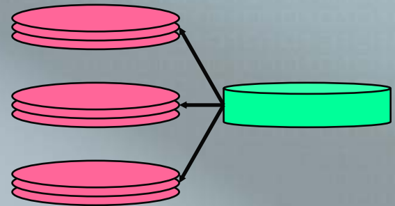
Volume RAID-5
