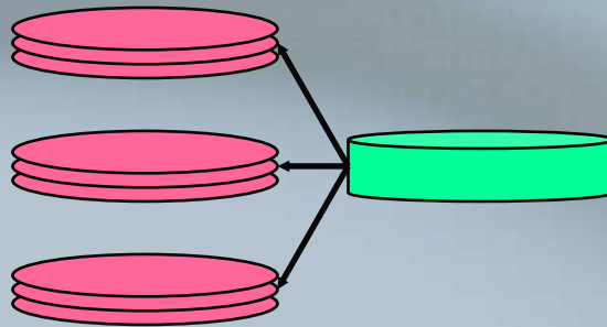
Volume RAID-5
