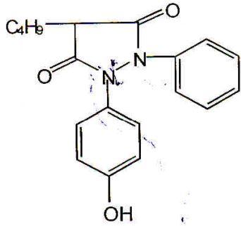
Oxyphenbutazone
