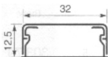
Sans cloison centrale
