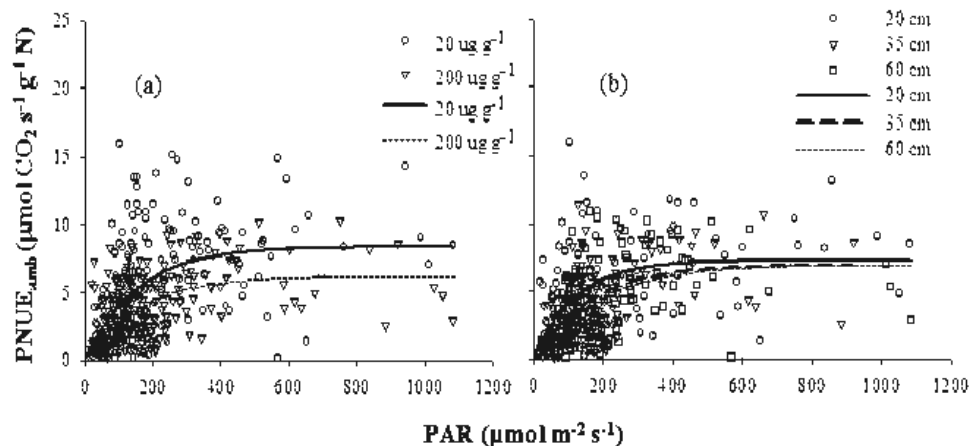
Figure 3.5 Photosynthetic N-use efficiency under ambient light conditions ( \text{PNUE}_{\text{amb}} )-photosynthetically active radiation (PAR) response curve under two nitrogen (N) levels (20 and 200 \mu\text{g g}^{-1} ) (a) and three spacings (20, 35, and 60 cm) (b) after 13 growing weeks. P < 0.001 and R^2 > 0.3 for all regressions.
