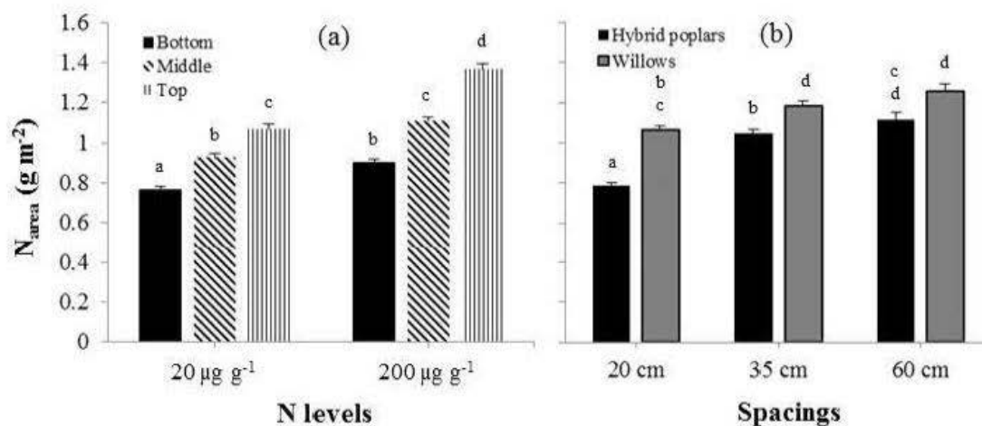
Figure 3.4 Mean nitrogen concentration ( N_{area} ) for each nitrogen levels (20 and 200 \mu g\ g^{-1} ) and crown section (bottom, middle, and top) (a) under three spacings (20, 35, and 60 cm) for hybrid poplars and willows (b) after 13 growing weeks. In each figure, means followed by the same letter do not significantly differ at \alpha = 0.05 .
