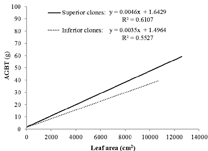
Figure 2.7 Relationship between leafless aboveground biomass per tree (AGBT) and leaf area for superior clones 2782, NM06, HAN-A5, SHE-E9, and TCH-N4 as a group and inferior clones 747210, 915319, LEV-D5, and LAF-I4 as a group after 13 growing weeks.
