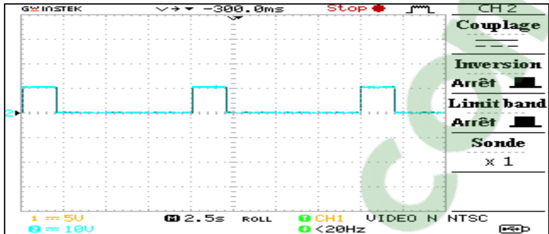
Figure III.14 : Signal Q3.
