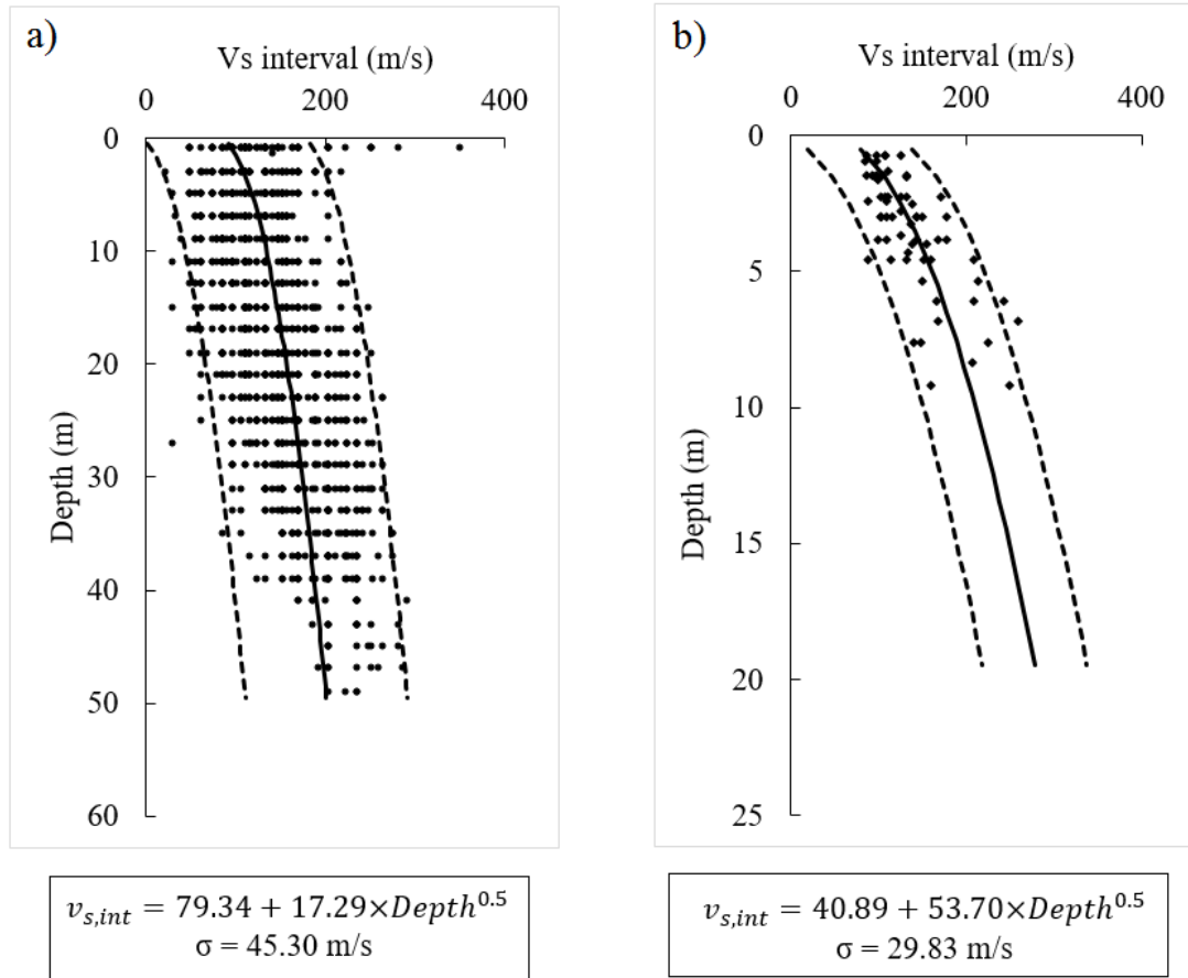
Figure 14 : Interval shear wave velocity vs depth relationship for a) clays, and b) sandy soils. Bold lines indicate average values; dashed lines indicate \pm 2 standard deviations ( \sigma )
